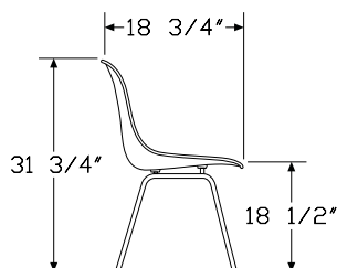
4-Leg Base
