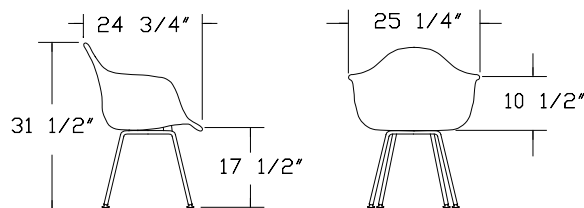
4-Leg Base
