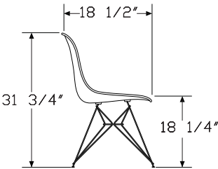
Wire Base
