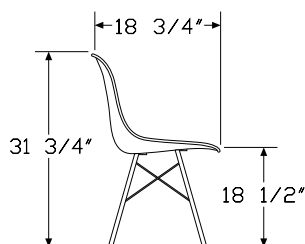
Dowel-Leg Base
