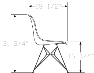
Wire Base
