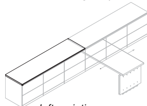
left variation (mortise stops on left, runs through on right)
