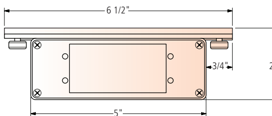
Front Elevation
