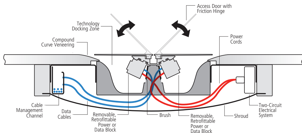
Power Block
