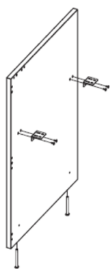
CLOSING SIDE PANEL
