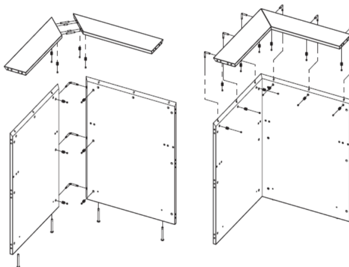
RECEPTION UPPER MODULE
