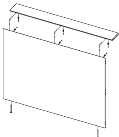
CLOSING SIDE PANEL
