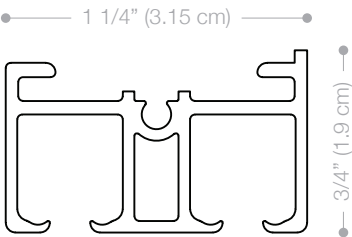
Two Channel Profile
