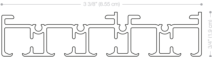
Five Channel Profile
