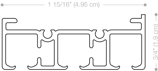
Three Channel Profile
