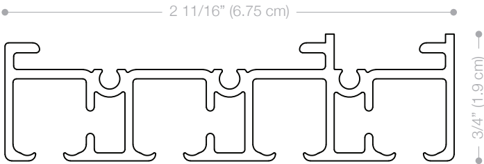
Four Channel Profile
