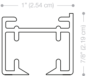
One Channel Profile* *Please note that One Channel track does not include end caps
