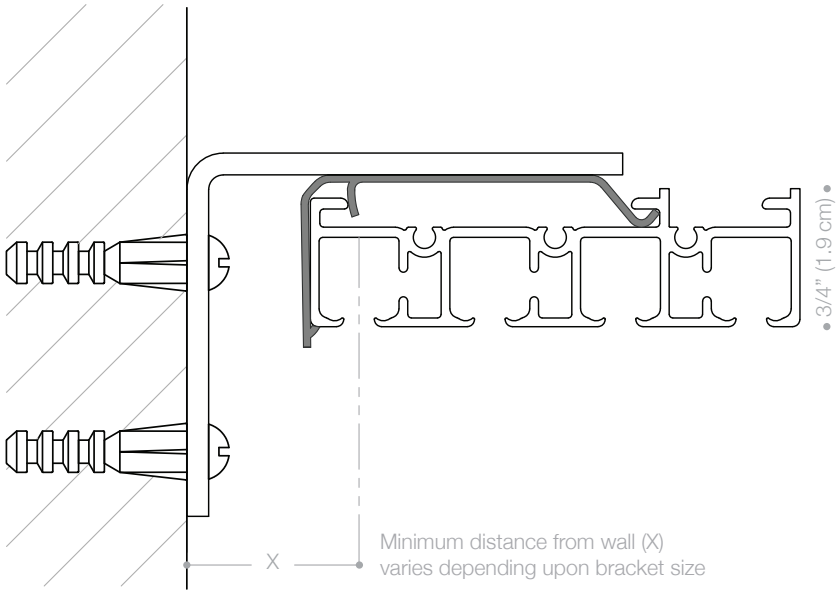
Wall Mounted Section
