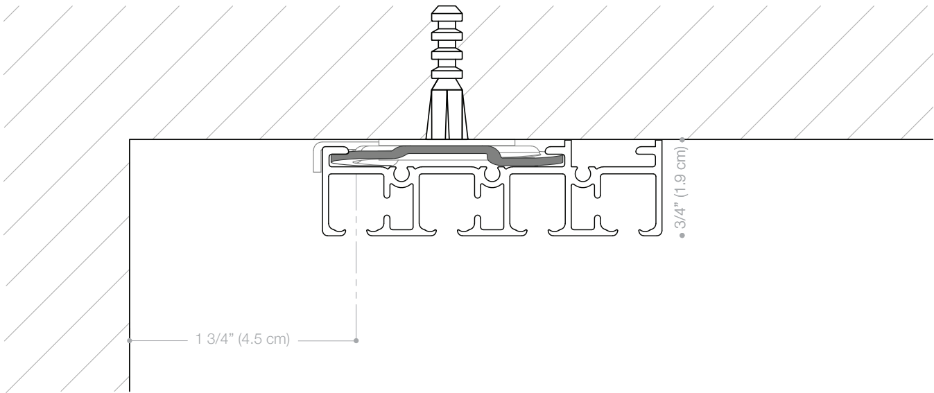
Ceiling Surface Mounted Section
