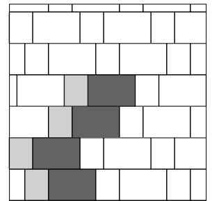
GR 057-001 33% /m² 40 x 30 cm / 16 x 12 inch 67% /m² 40 x 60 cm / 16 x 24 inch
