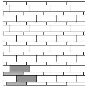
GR 016-002 33% /m² 10 x 60 cm / 4 x 24 inch 67% /m² 20 x 60 cm / 8 x 24 inch
