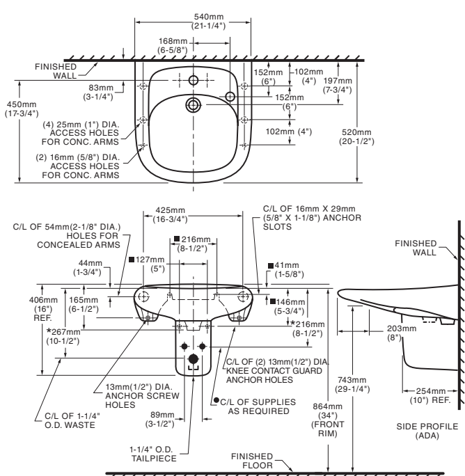
0955.123EC Center Hole With Extra Right Hand Hole
