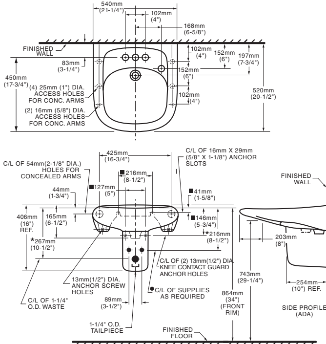
0954.123EC 4" Ctrs Extra Right Hand Hole
