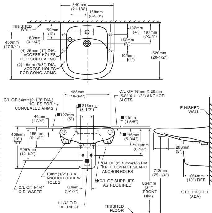
0955.121EC Center Hole With Extra Left Hand Hole
