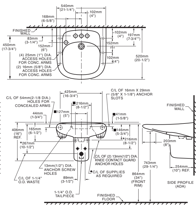
0954.121EC 4" Ctrs Extra Left Hand Hole
