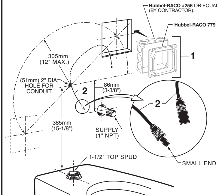
Fig.9 (TOP SPUD FIXTURE ILLUSTRATED)
