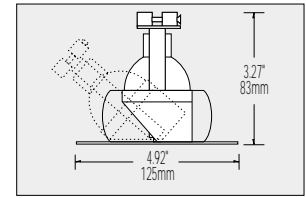
FDL-200RX - Round Adjustable
