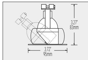
FDL-200R - Round Adjustable
