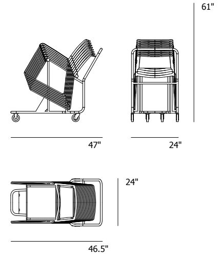
Four-wheeled trolley for 16 multipurpose chairs
