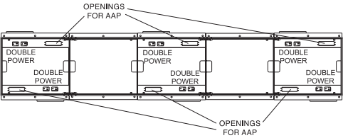
60" DataPath Tech Unit – Front View
