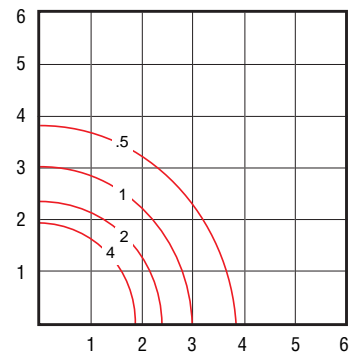
42w Fluorescent 3,200 Initial Lamp Lumens 0.90 Maintenance Factor
