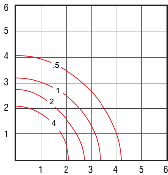
70w HPS 6,300 Initial Lamp Lumens 0.80 Maintenance Factor
