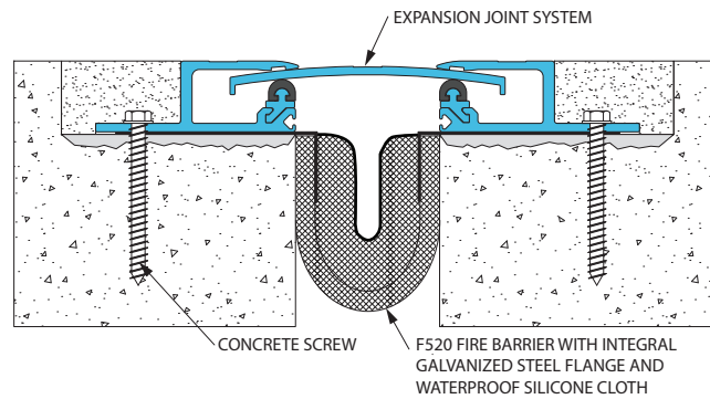
Top (Flush) Mount - Floor to Floor (300-A01-100 System Shown)
