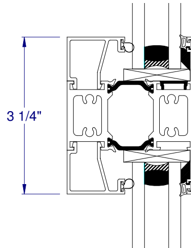
⑧ HORIZONTAL INTEGRAL FIXED/FIXED MULLION
