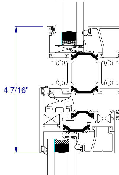
⑥ HORIZONTAL INTEGRAL FIXED/VENT MULLION
