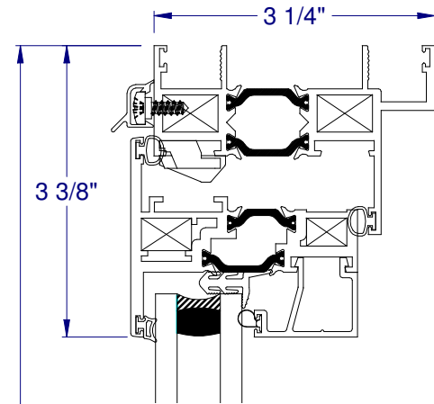
① HEAD VENT
