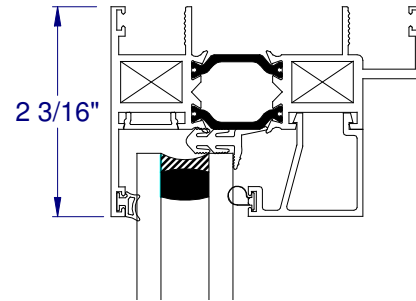
④ FIXED HEAD
