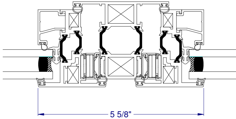
⑦ VERTICAL INTEGRAL VENT/VENT MULLION
