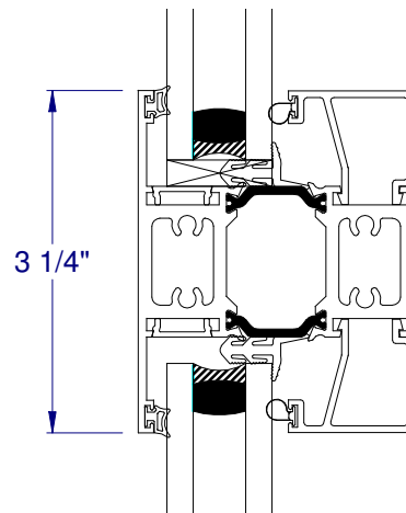
⑧ HORIZONTAL INTEGRAL FIXED/FIXED MULLION
