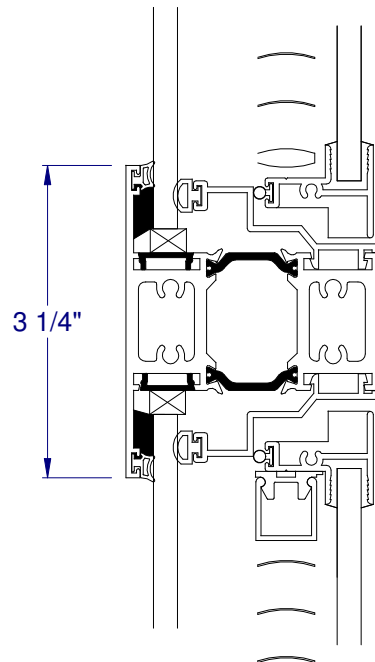
⑧ HORIZONTAL INTEGRAL FIXED/FIXED MULLION
