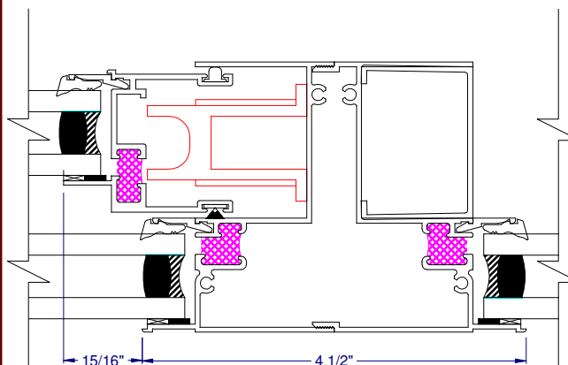
⑬ VERTICAL INTEGRAL MULLION (OPERABLE/FIXED)
