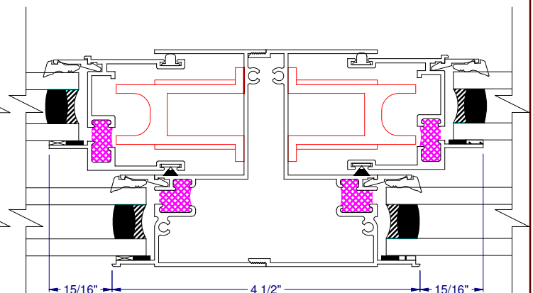
⑬ ALT. VERTICAL INTEGRAL MULLION (OPERABLE/OPERABLE)
