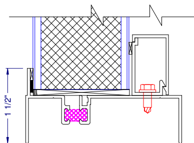
⑰ FIXED SILL (WITH 2" PANEL)
