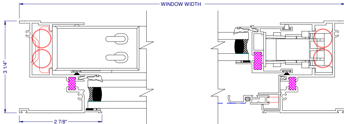
⑭ LEFT JAMB (WITH CLASS 5 BALANCES)
