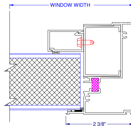
⑱ TRI-LIGHT FIXED JAMB (WITH 2" PANEL)
