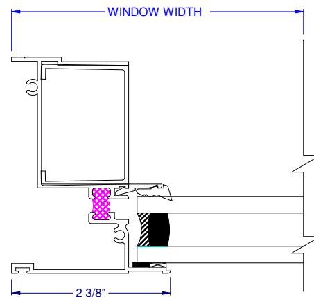
⑲ ALT. TRI-LIGHT FIXED JAMB (WITH ALTERNATE 1" INS. GLASS)
