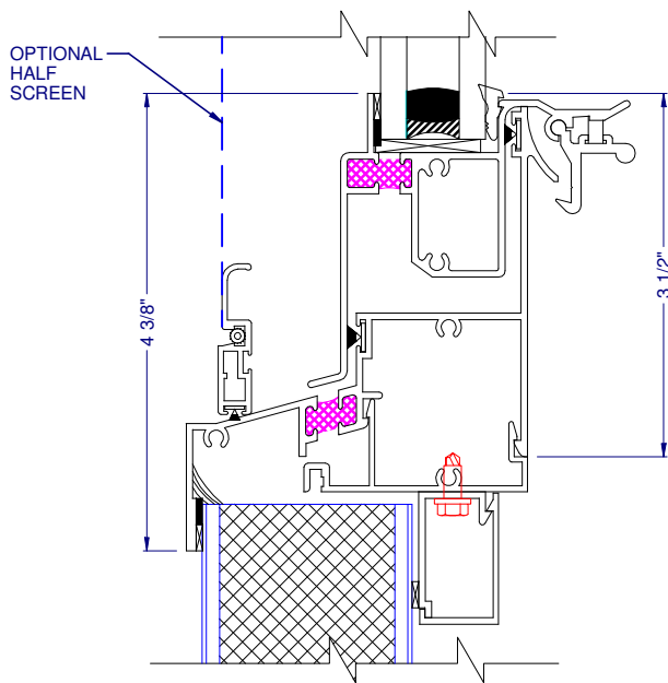
⑯ TRI-LIGHT INTERMEDIATE SILL (WITH 2" PANEL)
