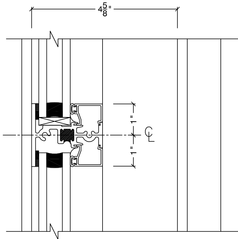
DETAIL-5
