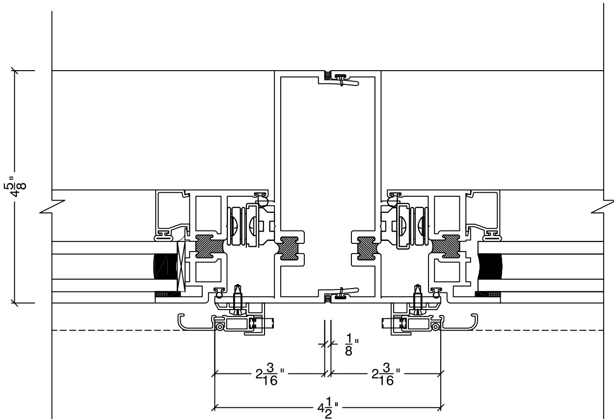
DETAIL-8
