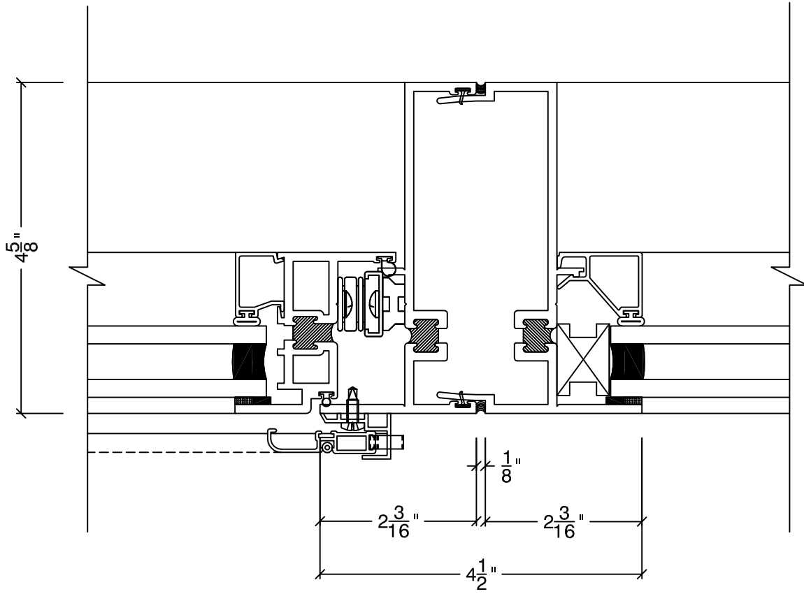
DETAIL-9
