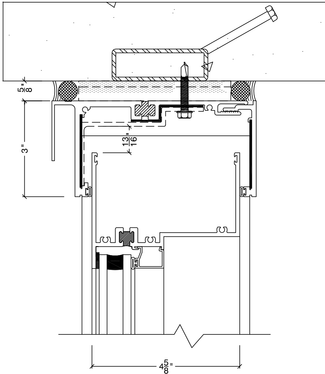
DETAIL-1
