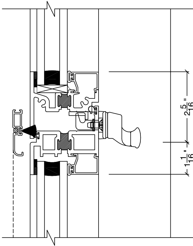
DETAIL-4
