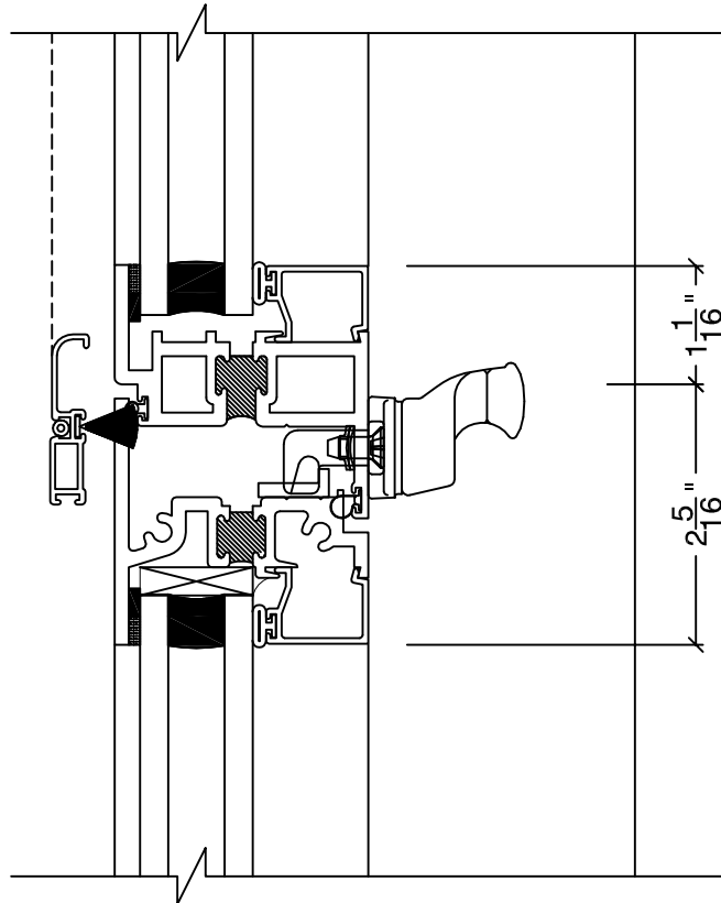
DETAIL-6
