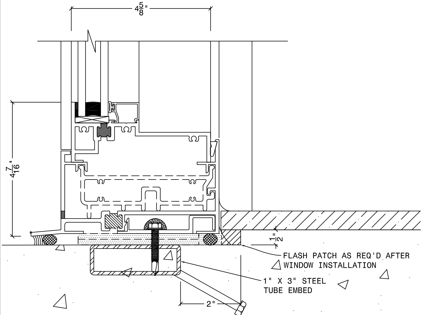
DETAIL-10
