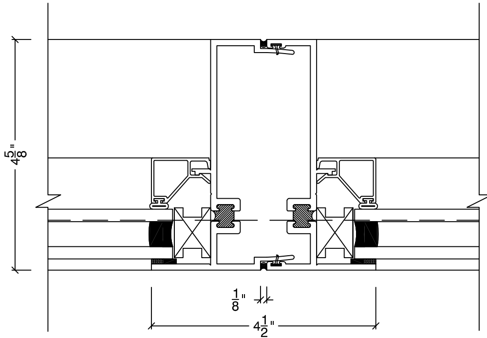
DETAIL-7
