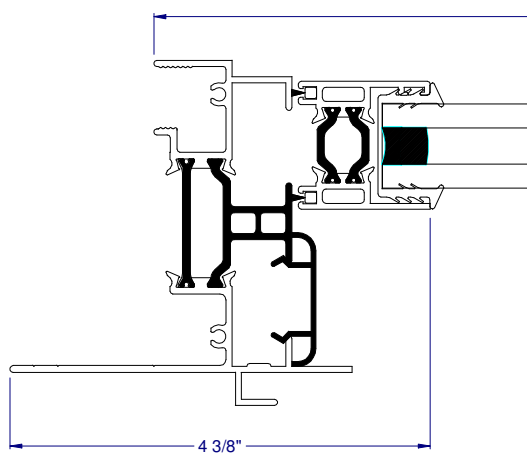
③A LEFT JAMB (FLANGE FRAME)
