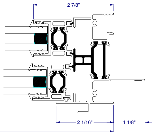
④B RIGHT JAMB (NAILFIN)
