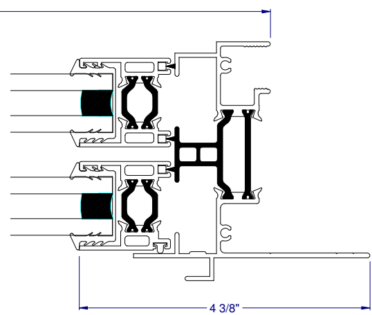
④A RIGHT JAMB (FLANGE FRAME)
