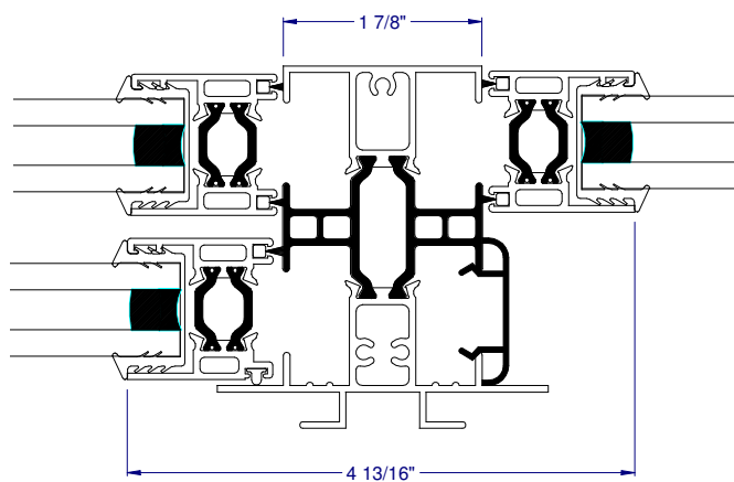
⑥ VERTICAL INTEGRAL MULLION
