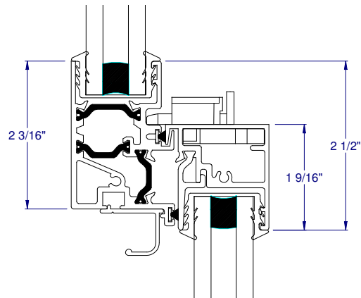
⑤ MEETING RAIL
