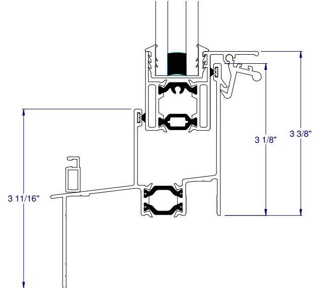
②B SILL (NAILFIN)
