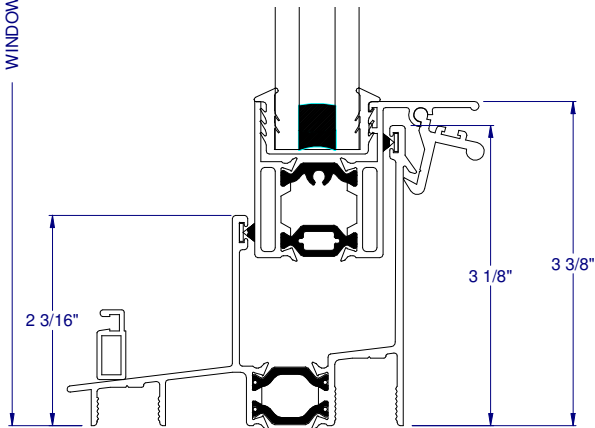
② SILL
