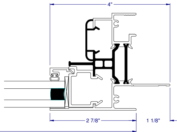
④B RIGHT JAMB (NAILFIN)
