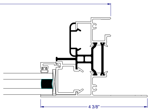
④A RIGHT JAMB (FLANGE)
