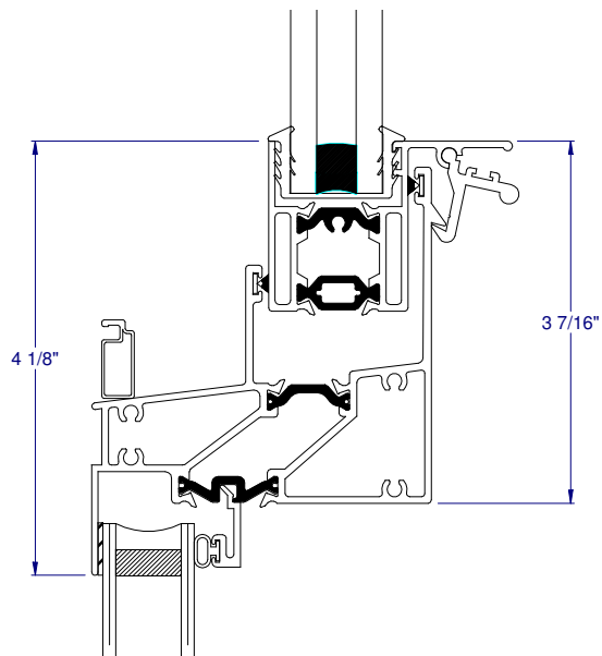
⑦ HORIZONTAL INTEGRAL MULLION
