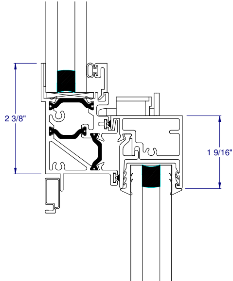
⑤ MEETING RAIL
