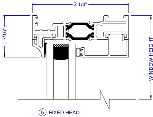
⑤ FIXED HEAD
