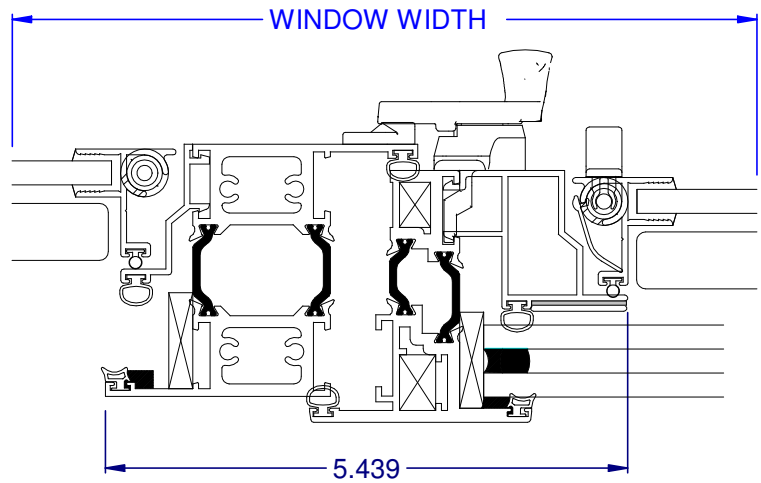
⑨ VERTICAL VENT/FIXED MULLION
