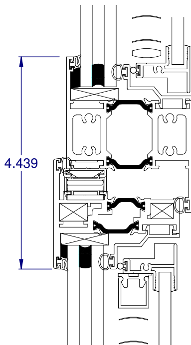
⑤ FIXED HEAD
