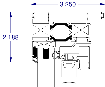
⑤ FIXED HEAD
