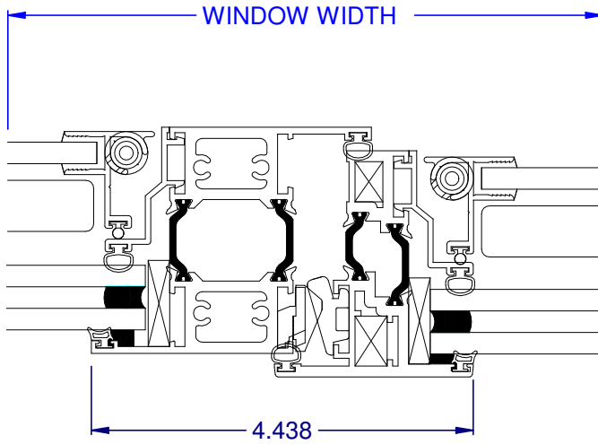
⑫ VERTICAL FIXED/VENT MULLION
