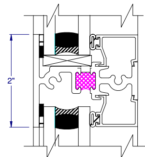
③③ TR-2800 HORIZ. INTEGRAL MULLION
