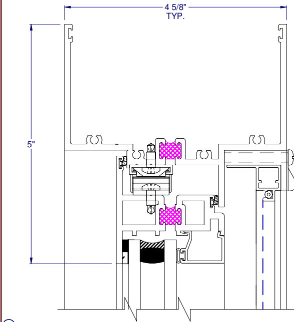
① VENT HEAD
