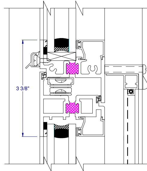
⑥ HORIZ. INTERGAL MULLION FIXED/VENT
