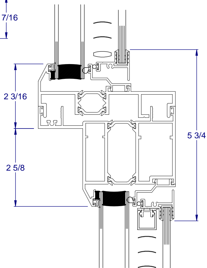
② SIMULATED MEETING RAIL
