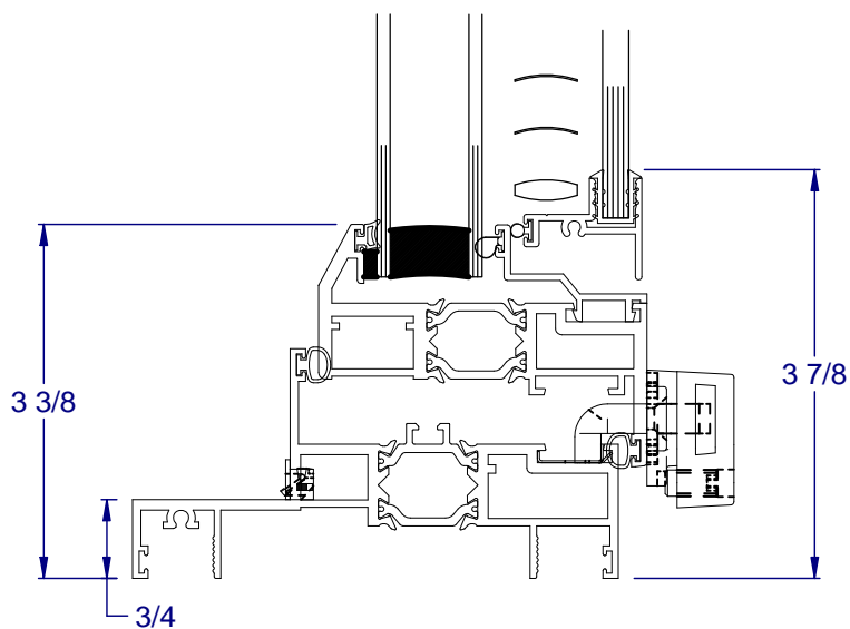
③ OPERABLE SILL
