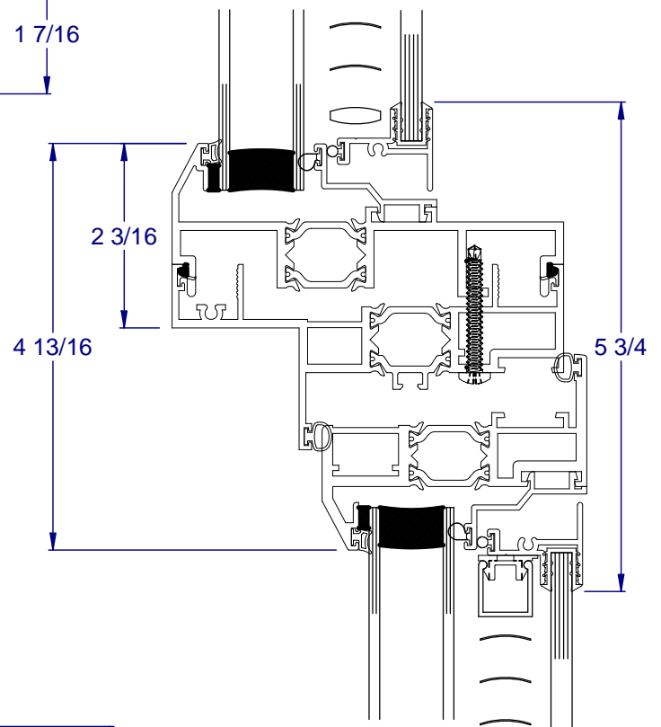
② SIMULATED MEETING RAIL
