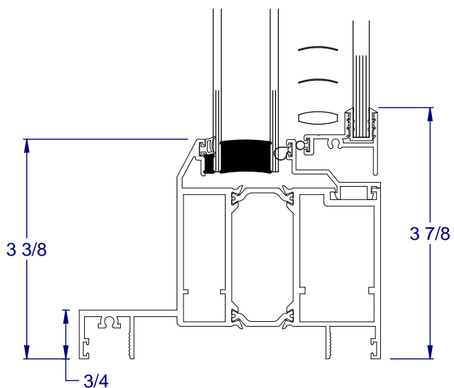
③ FIXED SILL
