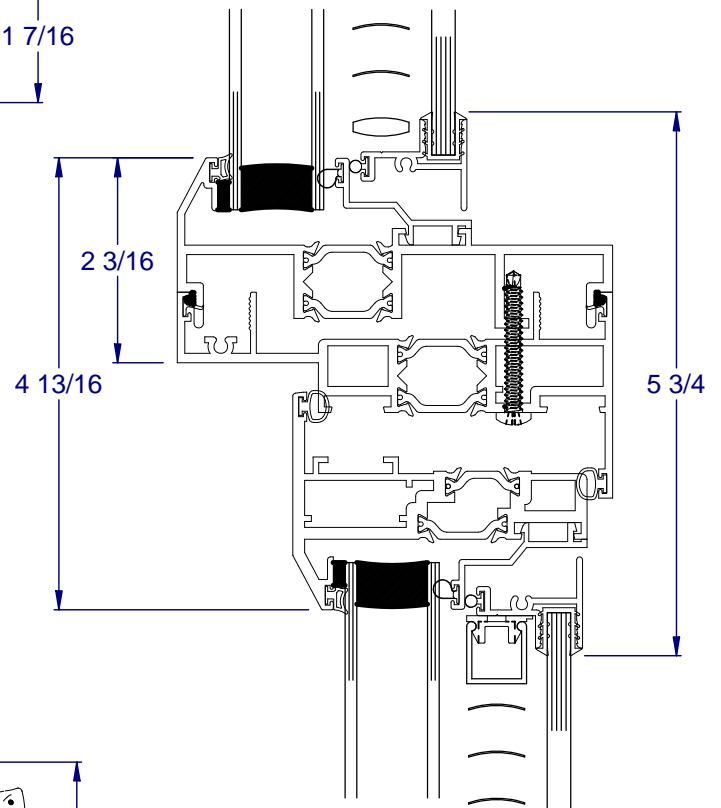
② SIMULATED MEETING RAIL
