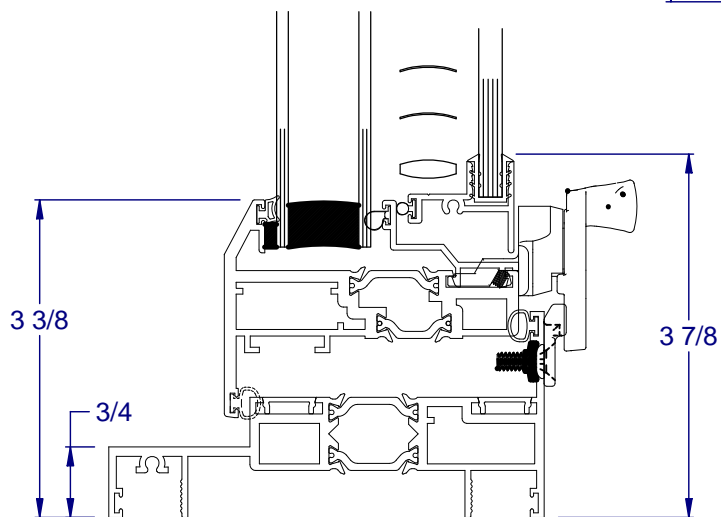
③ OPERABLE SILL
