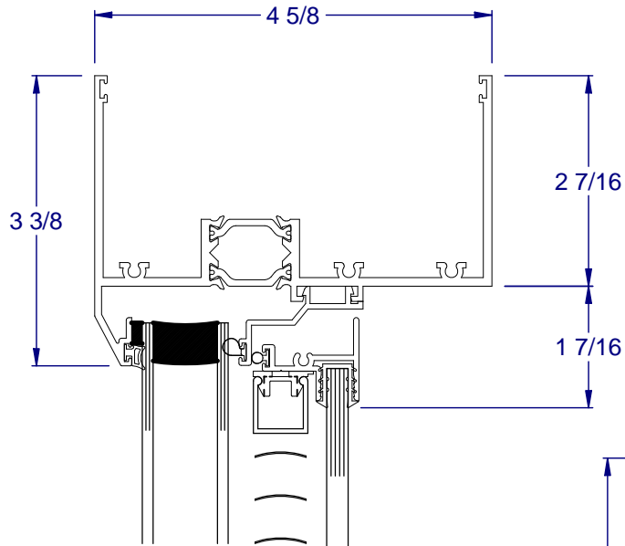
① FIXED HEAD
