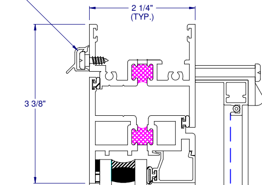
⑫ VENT HEAD
