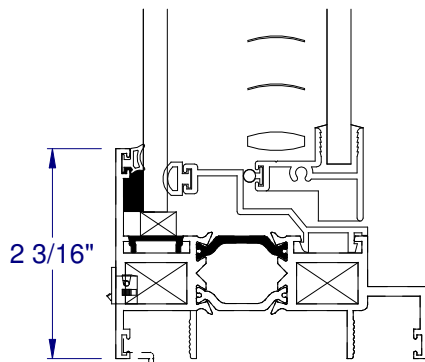
② FIXED SILL
