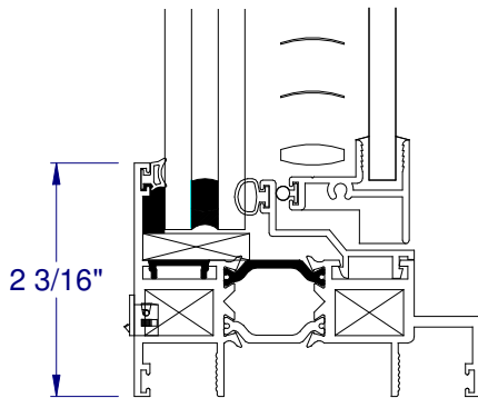
② FIXED SILL
