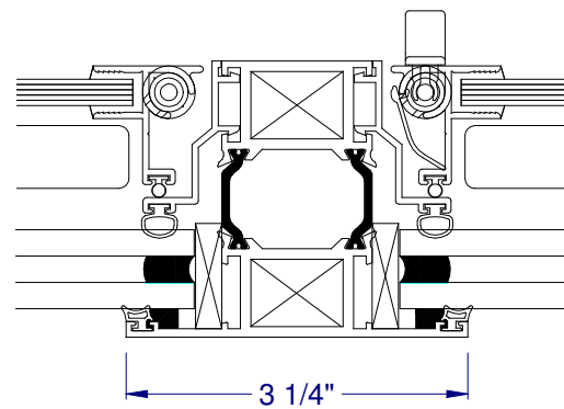
⑤ VERTICAL INTEGRAL FIXED/FIXED MULLION
