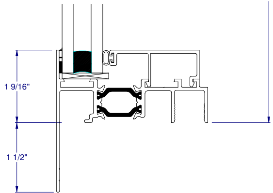
②A FIXED SILL (FLANGE FRAME)
