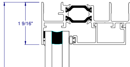
② FIXED SILL
