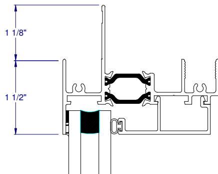
①B FIXED HEAD (NAILFIN)
