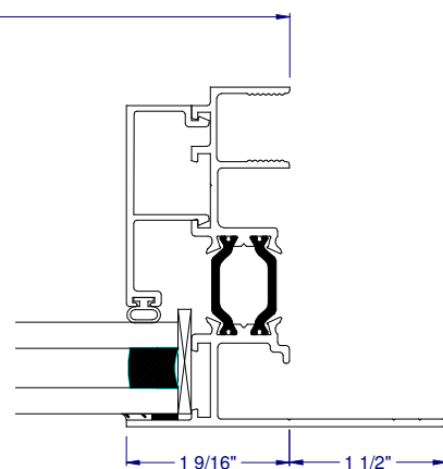
④A FIXED JAMB (FLANGE FRAME)
