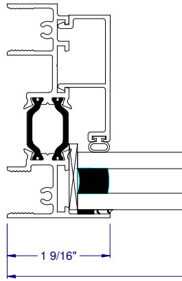
③A FIXED JAMB (FLANGE FRAME)
