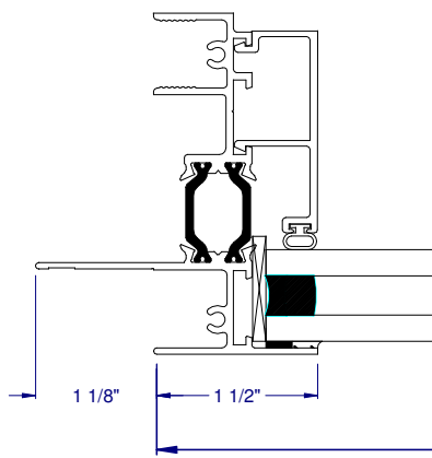
③B FIXED JAMB (NAILFIN)
