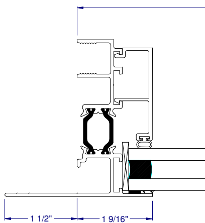
③A FIXED JAMB (FLANGE FRAME)
