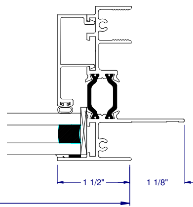
④B FIXED JAMB (NAILFIN)
