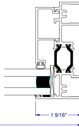
④A FIXED JAMB (FLANGE FRAME)
