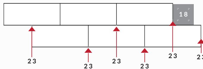
FIG. C: BELOW EYE LEVEL, USE #23 GAUGE NAILS, NAILING AT AN UPWARD ANGLE TO AVOID VISIBLE NAILS.
