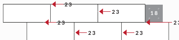
FIG. B: AT EYE LEVEL, USE #23 GAUGE NAILS, NAILING INTO THE EDGES OF EACH PANEL.
