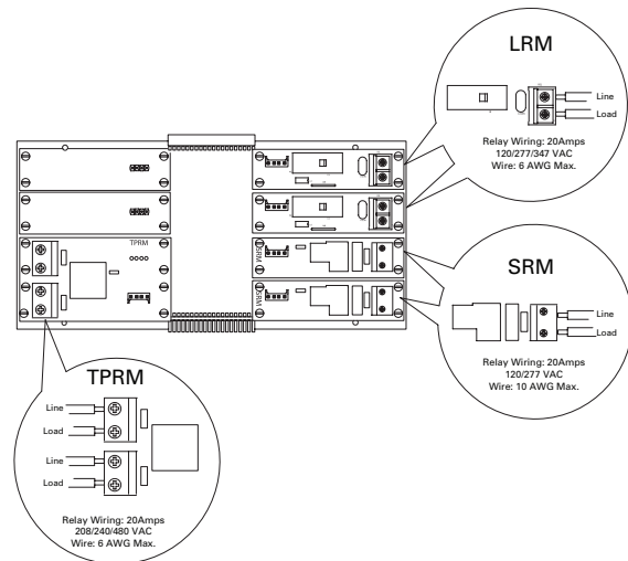
Modular Relay Card
