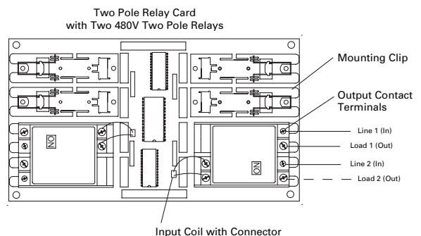
Two Pole Relay Card Wiring
