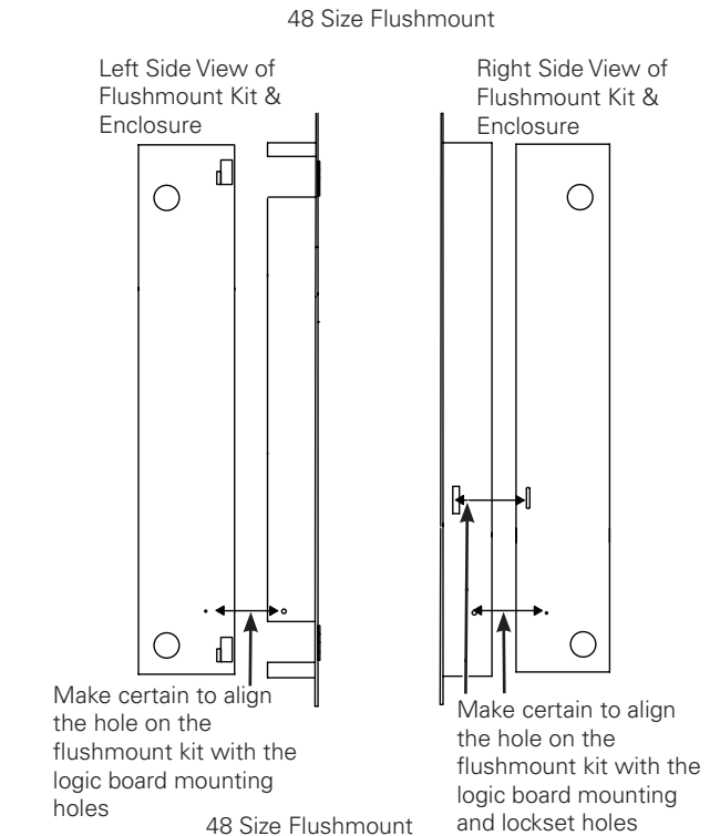
Figure 3. 48 Size Enclosure
