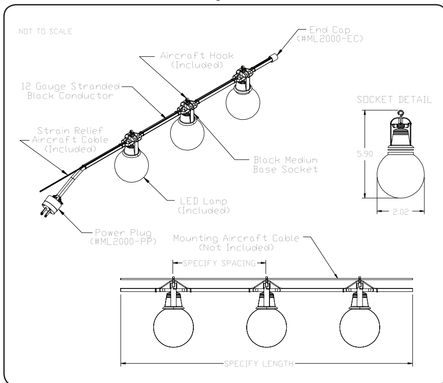
Drawing # ML1IN
