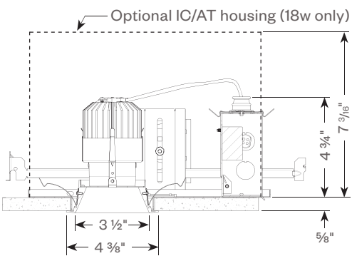
Ceiling Cutout Dimension: 4" dia.
