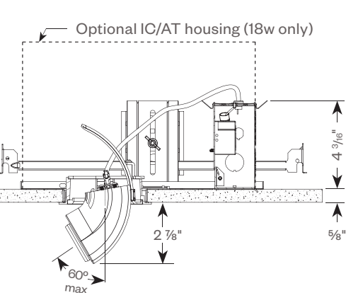
Ceiling Cutout Dimension: 4" dia.
