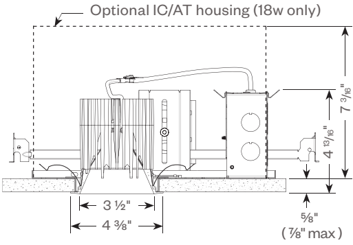
Ceiling Cutout Dimension: 4" dia.
