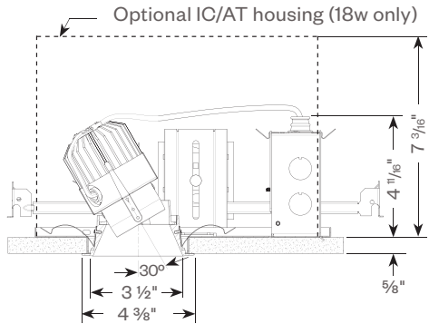
Ceiling Cutout Dimension: 4" dia.
