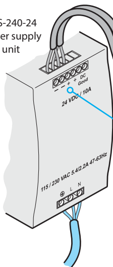
Mains input (115-230VAC 47-63Hz)
