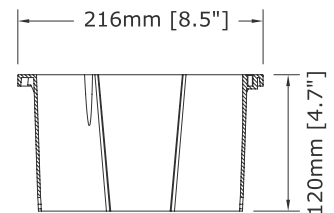
Inground Sleeve
