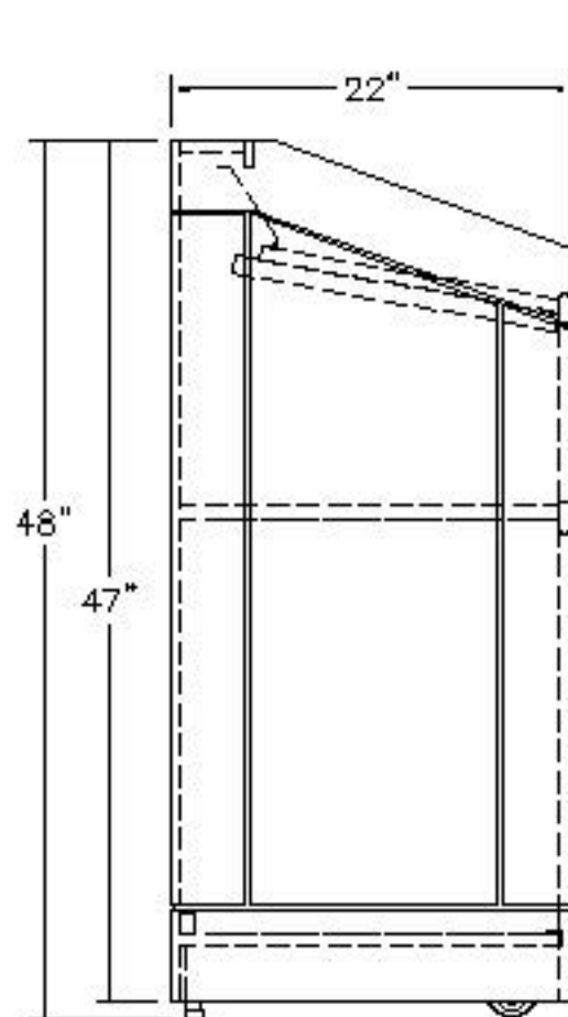
SIDE VIEW
