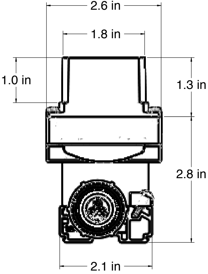
C6X 2FT MODULE w/ 1" LOUVERED LENS FRAME
