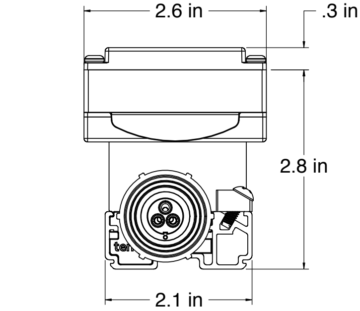
C6X 2FT MODULE w/ STANDARD LENS FRAME
