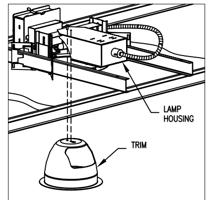
5.) CONNECT THE TRIM TO THE LAMP HOUSING AND TIGHTEN THE SCREW UNTIL TRIM IS FLUSH WITH CEILING. (TRIMS ARE ORDERED AND PACKED SEPARATELY) REFER TO RELAMP LABEL AND INSTALL PROPER LAMP/S.
