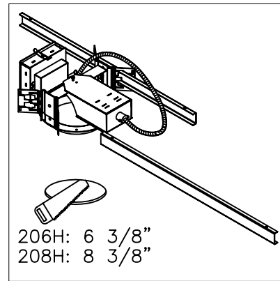
2.) INSTALL HANGER BARS (C-CHANNEL, NAILER BARS, CONDUIT, ETC...) (BY OTHERS OR CONSULT FACTORY)
