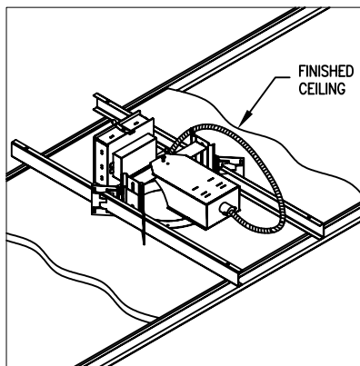
3.) SUPPORT FIXTURE BY THE HANGER BARS. SECURE HANGER BARS ACCORDING TO LOCAL BUILDING CODE. LOOSEN WING NUTS TO ADJUST BRACKETS SO BOTTOM OF FIXTURE FLANGE IS \frac{1}{8} " ABOVE THE FINISHED CEILING HEIGHT.
