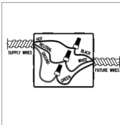
4.) MAKE SURE CIRCUIT IS NOT ENERGIZED AND MAKE SPLICES AS SHOWN. J-BOX IS SUITABLE FOR THRU WIRING ( 4 IN AND 4 OUT).
