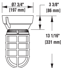
SURFACE MOUNT EMH
