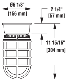
SURFACE MOUNT CFL & INC
