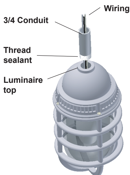
FIGURE 4 "- P -" PENDANT MOUNT MODEL
