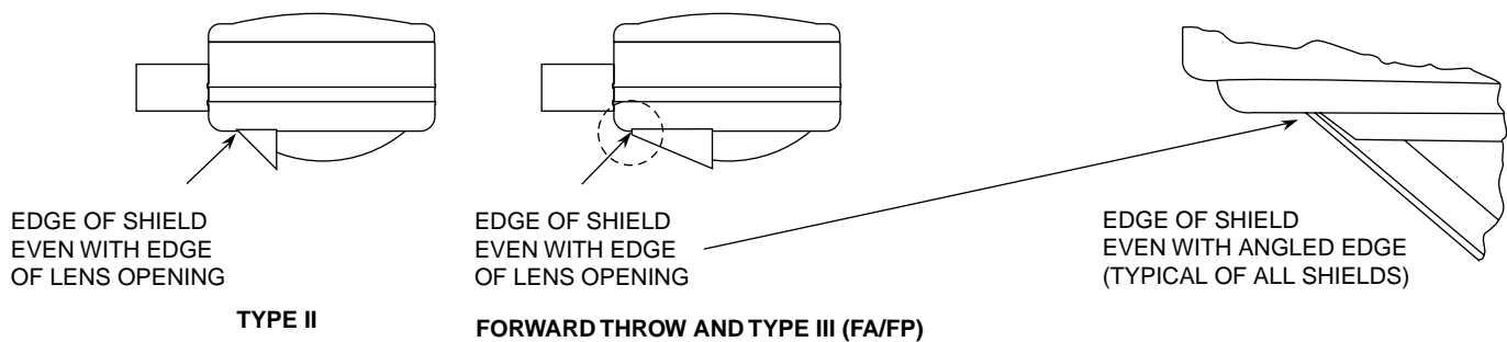
FIGURE 2: SHIELD POSITIONING
