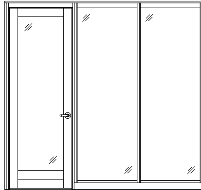
Elevation C
